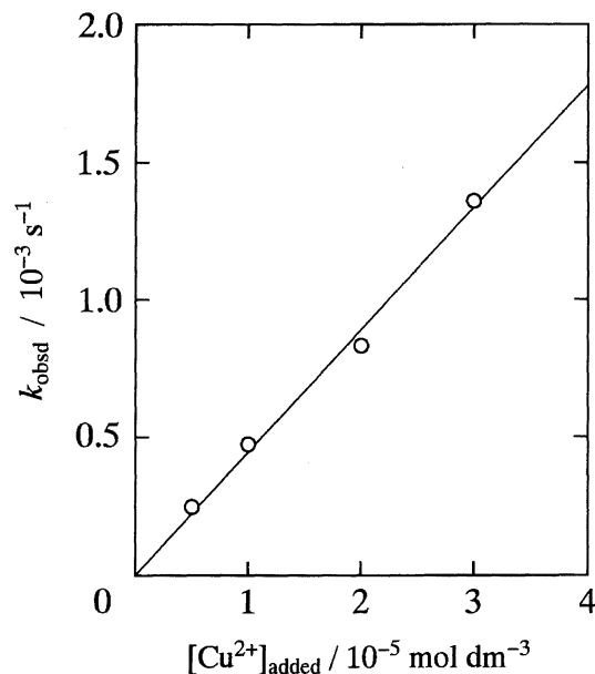
Fig. 6. Plots of k_{\text{obsd}} vs. [\text{Cu}^{2+}]_{\text{added}} for the decomposition of PDP under the same conditions as in Fig. 5. The solid line is the least-square's fit.
